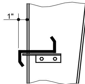
Inset Girt (Endwall Standard)
