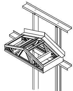
Walkdoor Canopy
