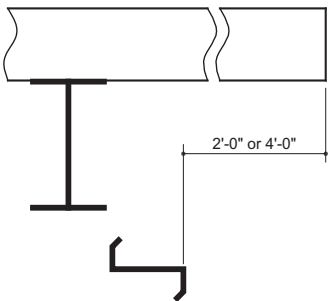
Rake Extension
