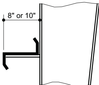
Bypass Girt (Sidewall Standard)
