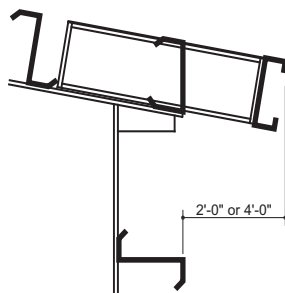
Eave Extension
